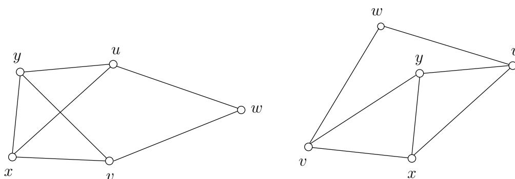
Figure 2: Two equivalent realizations of the rigid graph G of Figure 1, which show that the pair \{u, v\} is not globally linked in G .
