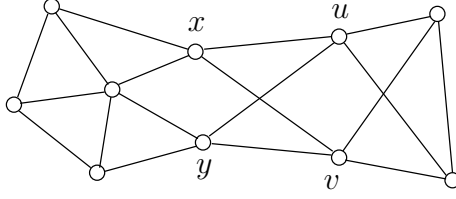
Figure 3: An M -circuit G obtained from a ‘wheel’ on six vertices and two copies of K_4 by taking 2-sums. The identified pairs of vertices, \{u, v\} and \{x, y\} , are globally linked in G .
