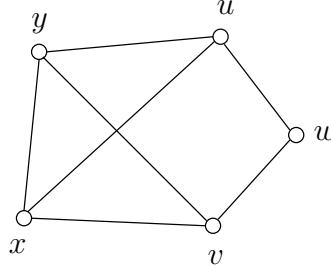
Figure 1: A realization (G, p) of a rigid graph G . The pair \{u, v\} is globally linked in (G, p) .
